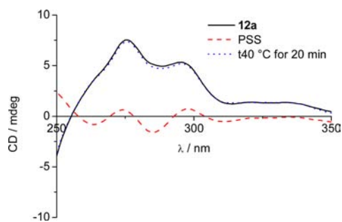
Figure 8. CD spectra of 12a (full line) and the mixture of 12a and 12b obtained after 10 s irradiation at 532 nm (dashed line) and the mixture after the thermal step (dotted line). Note that the opposite stereoisomer is used compared with 1 (Figure 4).
